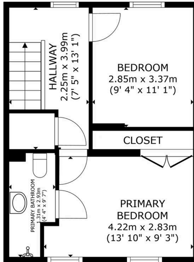
FLOOR 3
